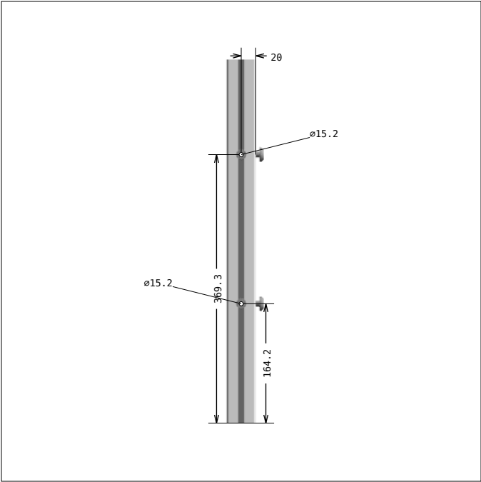
DRAWING 7, Pos 7 SIDE 3
