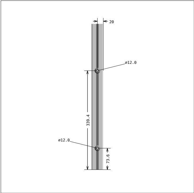
DRAWING 9, Pos 9 SIDE 2
