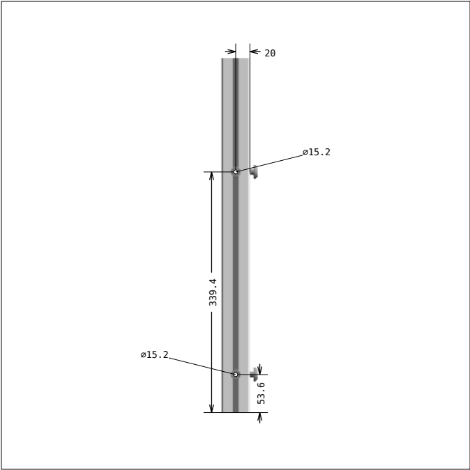
DRAWING 5, Pos 5 SIDE 3
