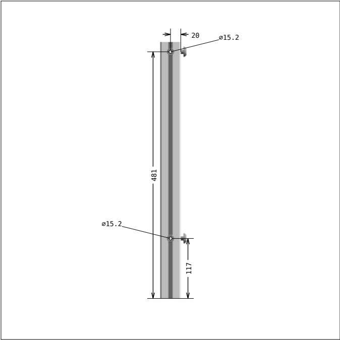
DRAWING 8, Pos 8 SIDE 3
