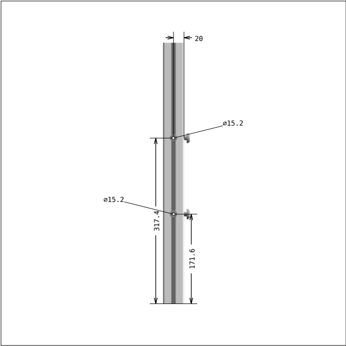
DRAWING 10, Pos 10 SIDE 3
