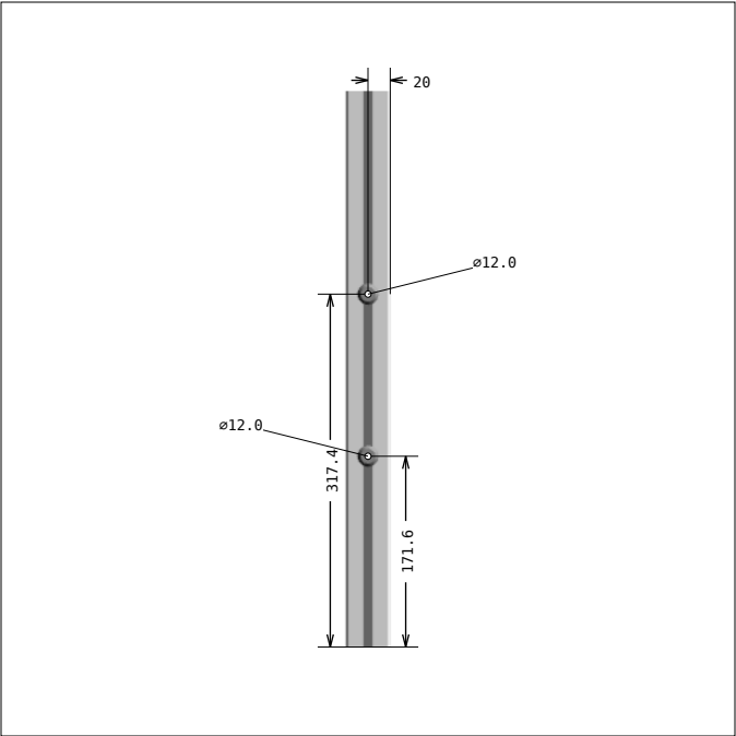
DRAWING 10, Pos 10 SIDE 2
