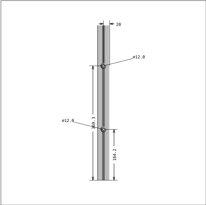
DRAWING 7, Pos 7 SIDE 2
