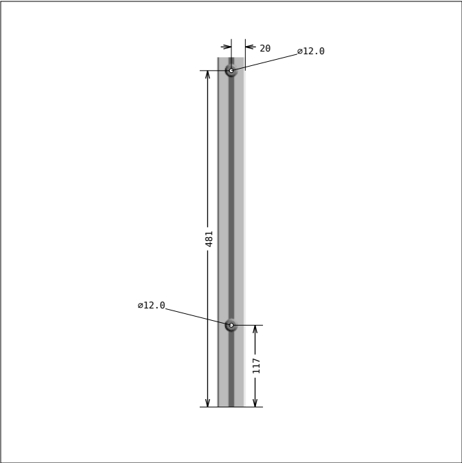
DRAWING 8, Pos 8 SIDE 2
