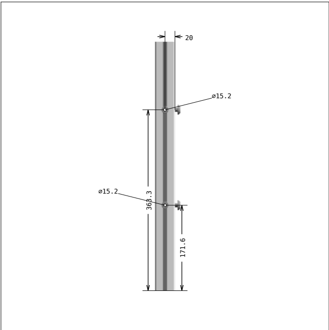
DRAWING 6, Pos 6 SIDE 3
