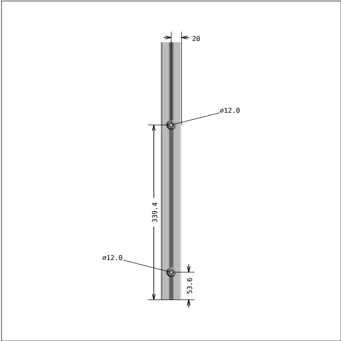
DRAWING 5, Pos 5 SIDE 2
